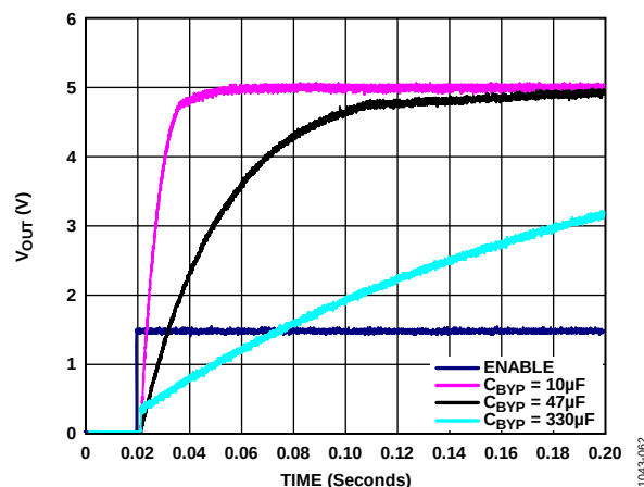
Figure 62. Typical Start-Up Behavior with C_{BYP} = 10\text{ }\mu\text{F} to 330\text{ }\mu\text{F}
