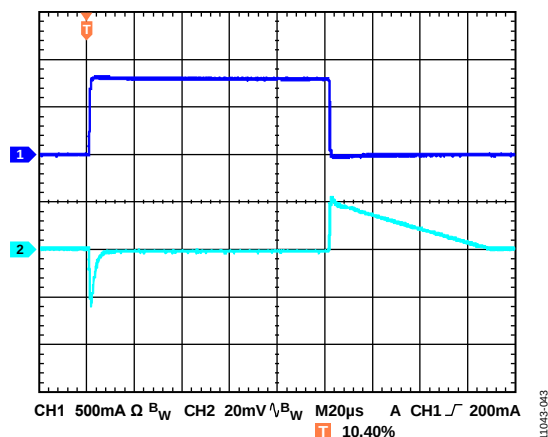
Figure 43. Load Transient Response, I_{LOAD} = 1 \text{ mA} to 800 \text{ mA} , V_{OUT} = 5 \text{ V} , V_{IN} = 6.2 \text{ V} , CH1 = I_{OUT} , CH2 = V_{OUT}
