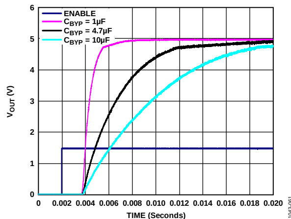
Figure 61. Typical Start-Up Behavior with C_{BYP} = 1\text{ }\mu\text{F} to 10\text{ }\mu\text{F}
