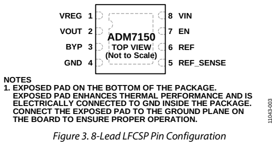
Figure 3. 8-Lead LFCSP Pin Configuration
