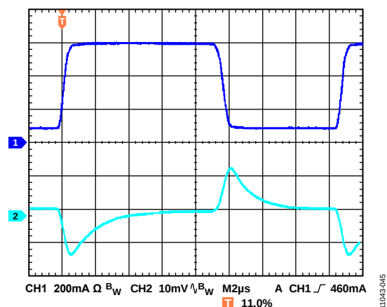
Figure 45. Load Transient Response, I_{LOAD} = 100 \text{ mA} to 600 \text{ mA} , V_{OUT} = 5 \text{ V} , V_{IN} = 6.2 \text{ V} , CH1 = I_{OUT} , CH2 = V_{OUT}
