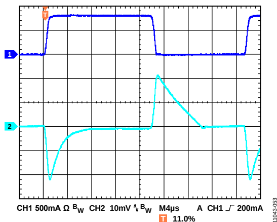
Figure 53. Output Transient Response, V_{\text{OUT}} = 5\text{ V} , C_{\text{OUT}} = 10\text{ }\mu\text{F} , CH1 = Load Current, CH2 = V_{\text{OUT}}
