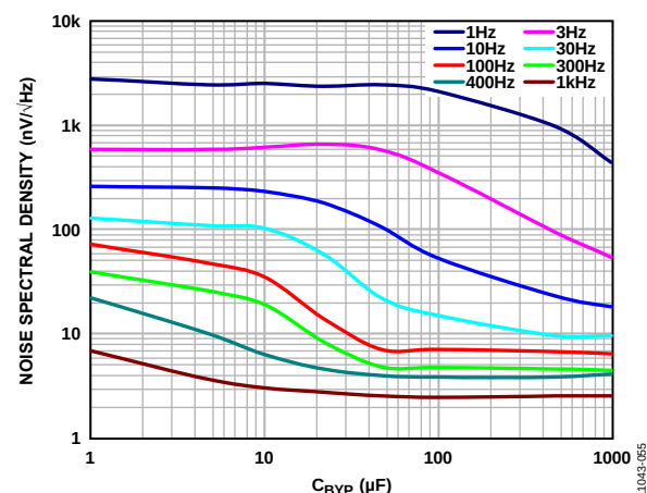
Figure 55. Noise Spectral Density vs. Capacitance ( C_{\text{BYP}} ) for Different Frequencies
