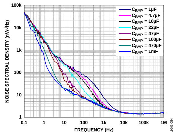
Figure 54. Noise Spectral Density vs. Frequency, C_{\text{BYP}} = 1\text{ }\mu\text{F} to 1 mF
