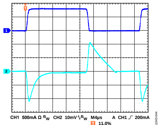
Figure 44. Load Transient Response, I_{LOAD} = 10 \text{ mA} to 800 \text{ mA} , V_{OUT} = 5 \text{ V} , V_{IN} = 6.2 \text{ V} , CH1 = I_{OUT} , CH2 = V_{OUT}
