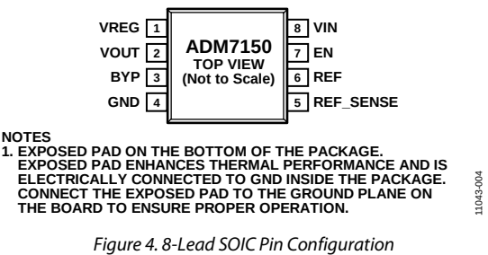
Figure 4. 8-Lead SOIC Pin Configuration
