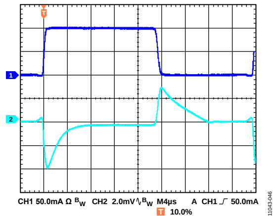
Figure 46. Load Transient Response, I_{LOAD} = 1 \text{ mA} to 100 \text{ mA} , V_{OUT} = 5 \text{ V} , V_{IN} = 6.2 \text{ V} , CH1 = I_{OUT} , CH2 = V_{OUT}
