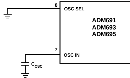
Figure 4b. External Capacitor
