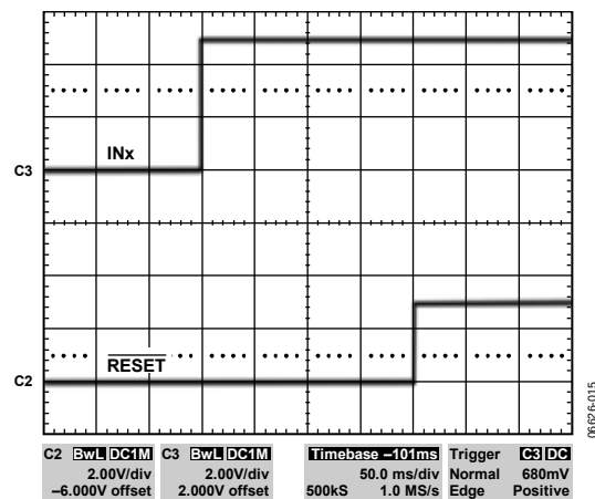
Figure 11. RESET Timeout Delay (50 ms/div)
