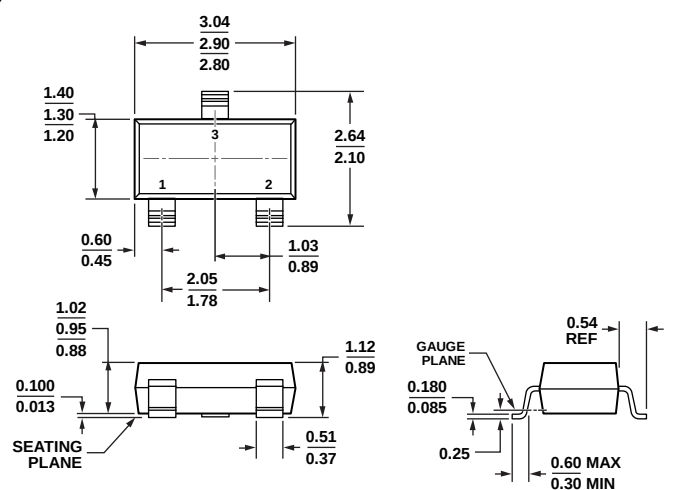
Figure 10. 3-Lead Small Outline Transistor Package [SOT-23-3] (RT-3) Dimensions shown in millimeters
