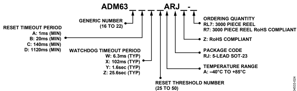
Figure 22. Ordering Code Structure (Modified Diagram)
