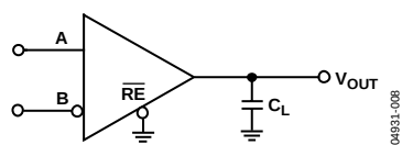
Figure 8. Receiver Propagation Delay
