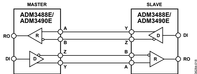
Figure 32. ADM3488E/ADM3490E Full-Duplex Point-to-Point Applications
