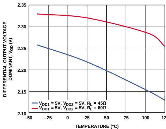
Figure 14. Driver Differential Output Voltage Dominant vs. Temperature
