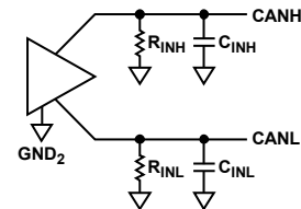
Figure 22. Input Resistance ( R_{INX} ) and Input Capacitance ( C_{INX} ) Measured in Recessive State, Bus Disconnected
