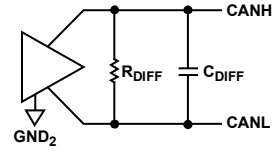
Figure 21. R_{DIFF} and C_{DIFF} Measured in Recessive State, Bus Disconnected
