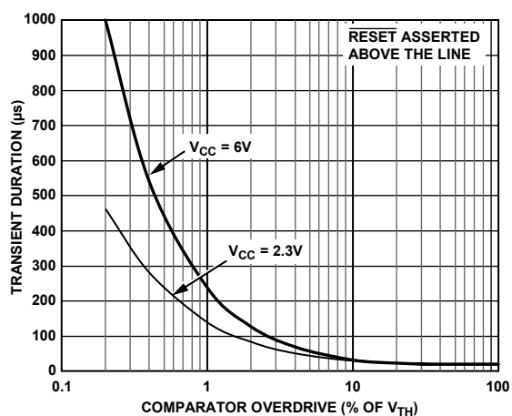
Figure 9. Transient Duration vs. Comparator Overdrive
