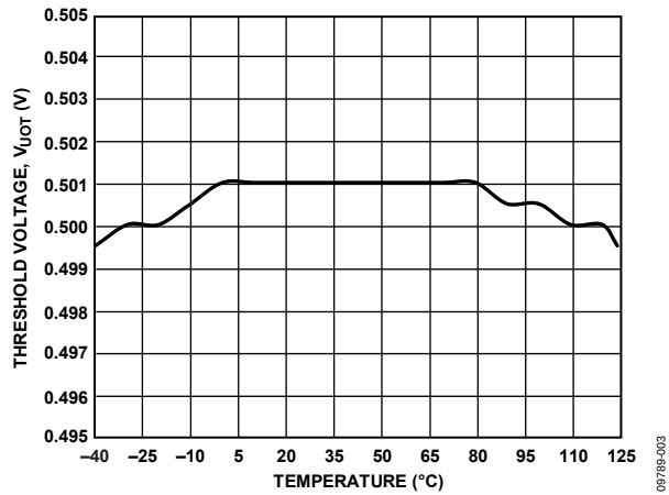
Figure 3. Input Threshold Voltage vs. Temperature
