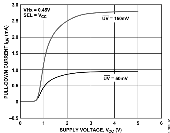
Figure 12. I_{SINK} , I_{UV} vs. V_{CC}
