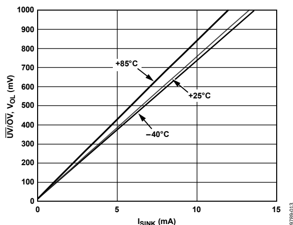
Figure 13. \overline{UV}/\overline{OV} Voltage Output Low vs. Output Sink Current
