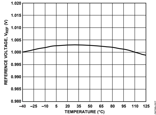
Figure 7. Buffered Reference Voltage vs. Temperature
