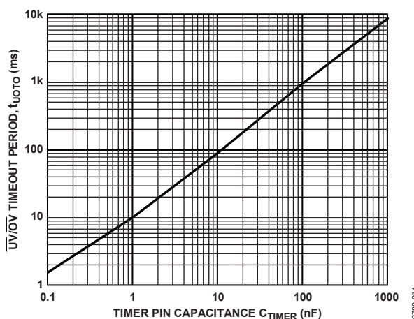
Figure 14. \overline{UV}/\overline{OV} Timeout Period vs. Capacitance
