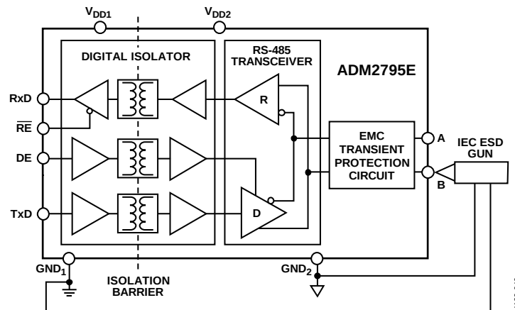
Figure 40. IEC 61000-4-2 ESD Testing to GND 1 or GND 2
