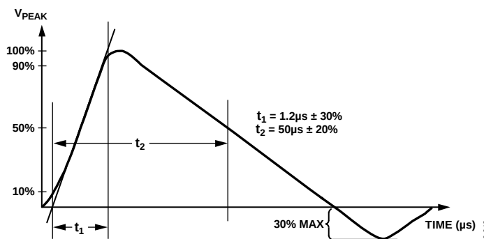
Figure 44. IEC 61000-4-5 Surge 1.2 \mu\text{s}/50 \mu\text{s} Waveform
