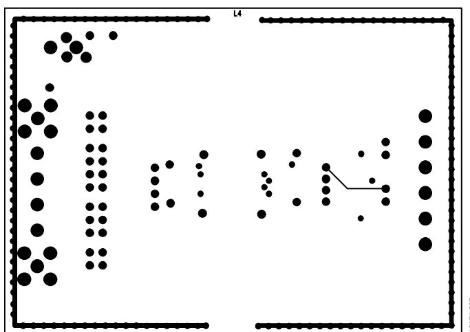
Figure 8. Internal Layer 4
