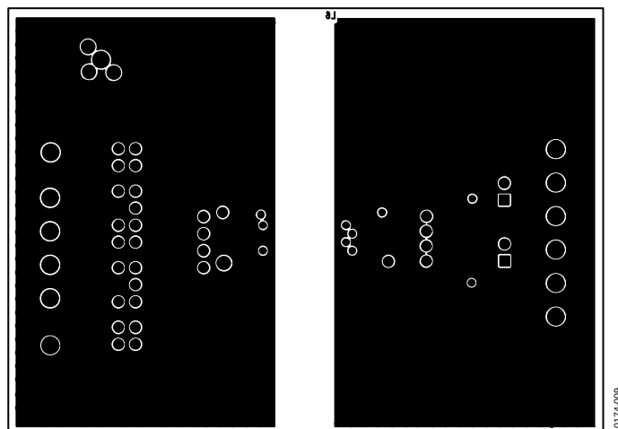
Figure 10. Bottom Solder Layer
