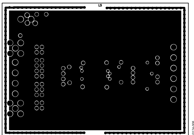
Figure 9. Internal Layer 5
