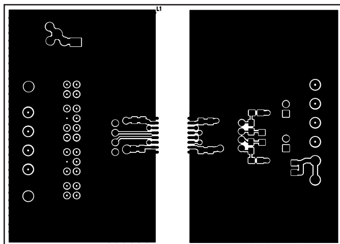
Figure 4. Top Layer
