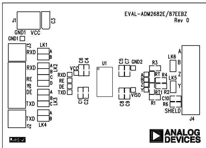
Figure 5. Silkscreen
