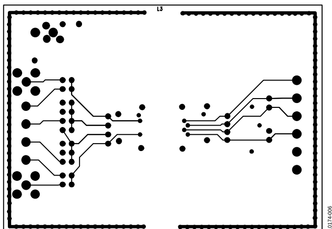
Figure 7. Internal Layer 3
