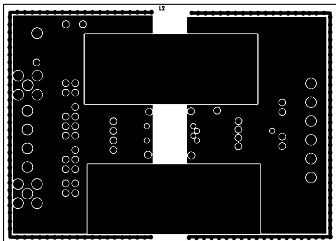
Figure 6. Internal Layer 2
