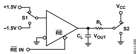
Figure 28. Receiver Enable/Disable
