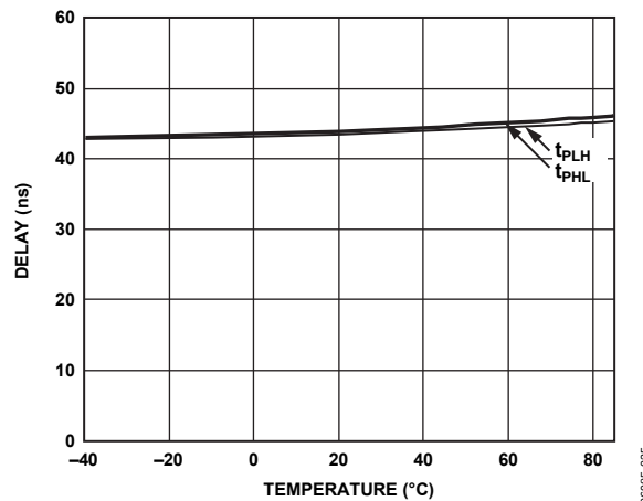
Figure 17. Receiver Propagation Delay vs. Temperature
