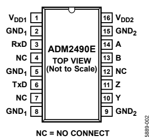
Figure 2. Pin Configuration
