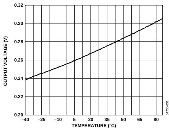
Figure 16. Receiver Output Low Voltage vs. Temperature, I = -4\text{ mA}
