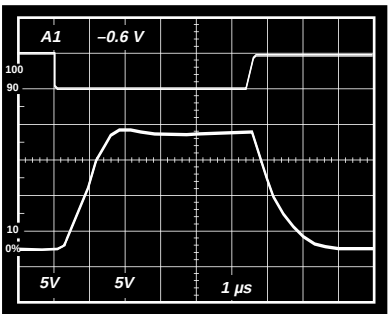
Figure 18. Transmitter Fully Loaded Slew Rate
