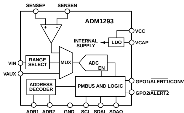
Figure 1. ADM1293 Functional Block Diagram
