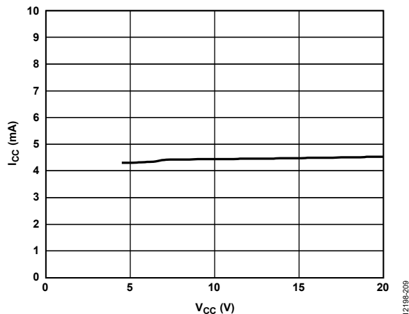
Figure 8. Supply Current ( I_{CC} ) vs. V_{CC}
