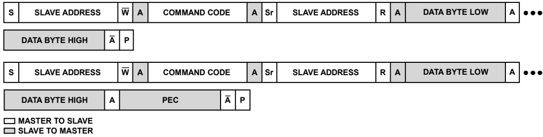
Figure 67. Read Word and Read Word with PEC
