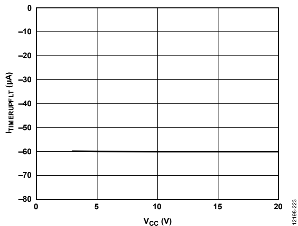
Figure 20. TIMER Pull-Up Current OC Fault ( I_{T\text{IMERUPFLT}} ) vs. V_{CC}
