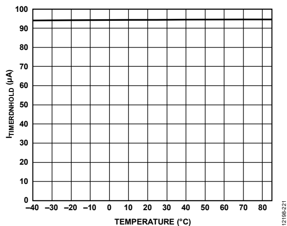
Figure 22. TIMER Pull-Down Current Hold ( I_{T\text{IMERDNHOLD}} ) vs. Temperature
