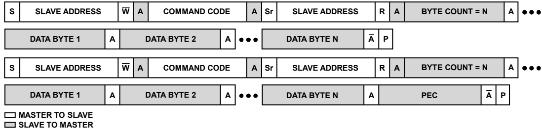
Figure 68. Block Read and Block Read with PEC
