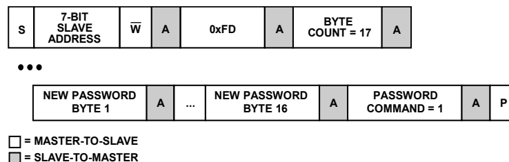
Figure 18. Block Write Command for Changing the Password
