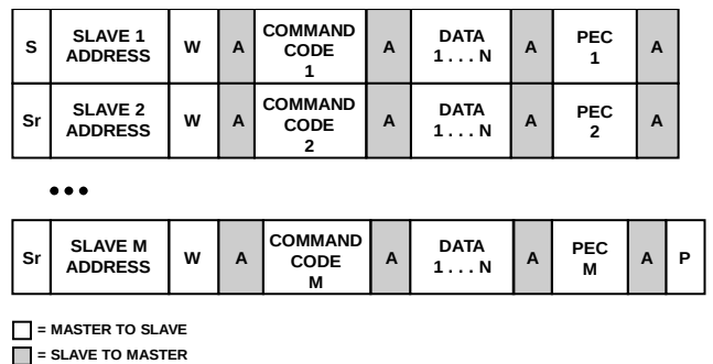
Figure 28. Group Command Protocol with PEC
