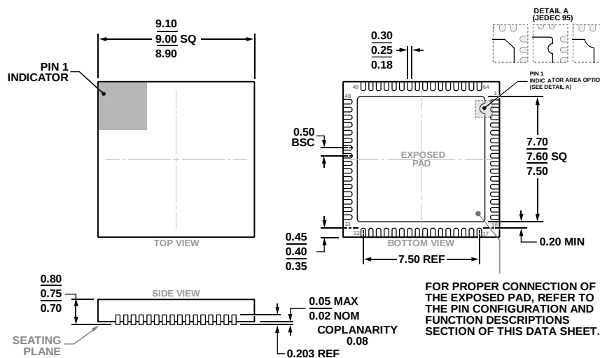
Figure 30. 64-Lead Lead Frame Chip Scale Package [LFCSP] 9 mm × 9 mm Body and 0.75 mm Package Height (CP-64-15)
