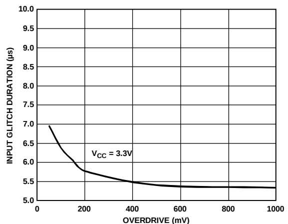
Figure 15. \overline{FAULT} Input Glitch Immunity vs. Input Overdrive
