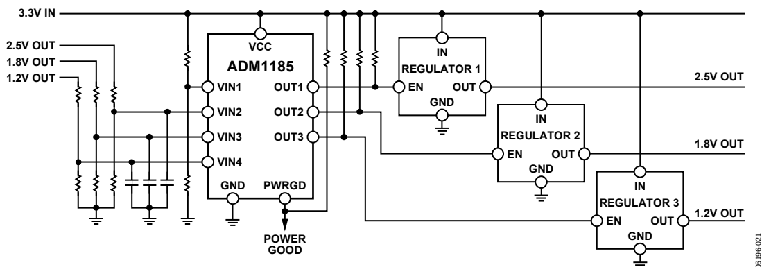
Figure 18. Voltage Monitoring and Sequencing Application Diagram
