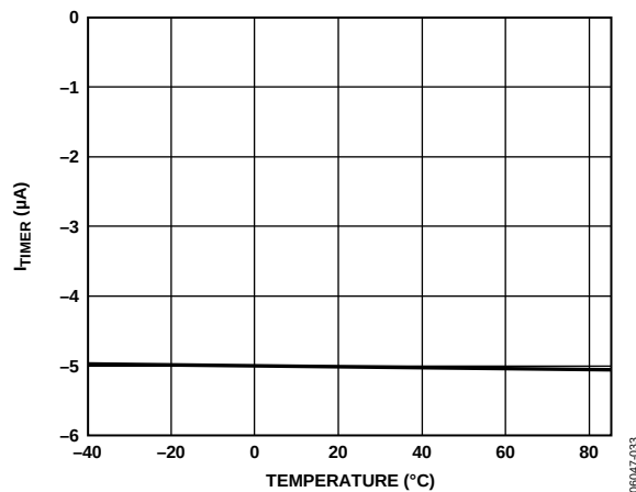
Figure 19. Timer Pull-Up Current (Initial Cycle) vs. Temperature
