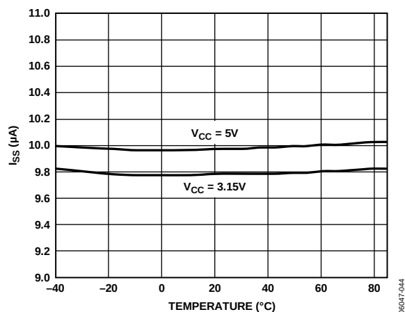
Figure 30. SS Pin Pull-Up Current vs. Temperature
