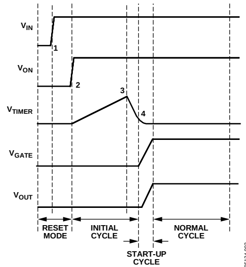
Figure 33. Power-Up Timing
