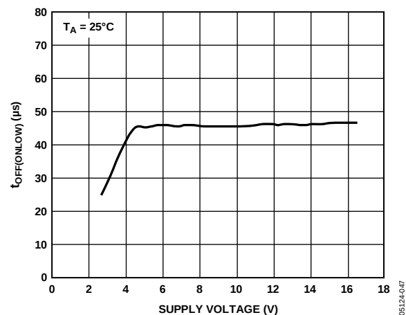
Figure 24. t_{\text{OFF}}(\text{ONLOW}) vs. Supply Voltage
