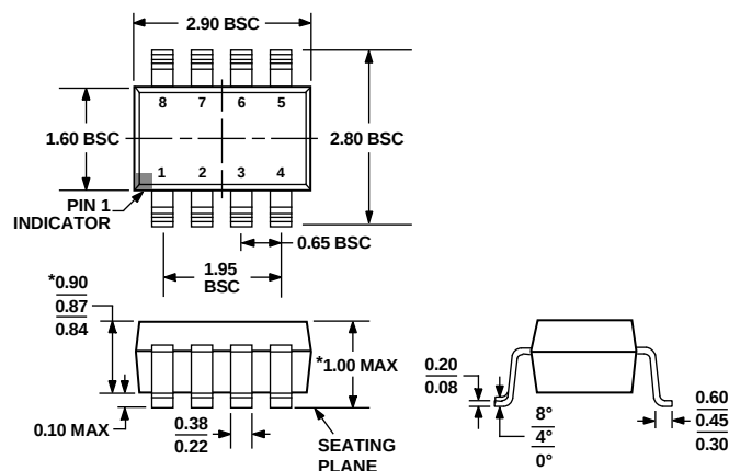
*COMPLIANT TO JEDEC STANDARDS MO-193-BA WITH THE EXCEPTION OF PACKAGE HEIGHT AND THICKNESS. Figure 37. 8-Lead Thin Small Outline Transistor Package [TSOT] (UJ-8) Dimensions shown in millimeters
