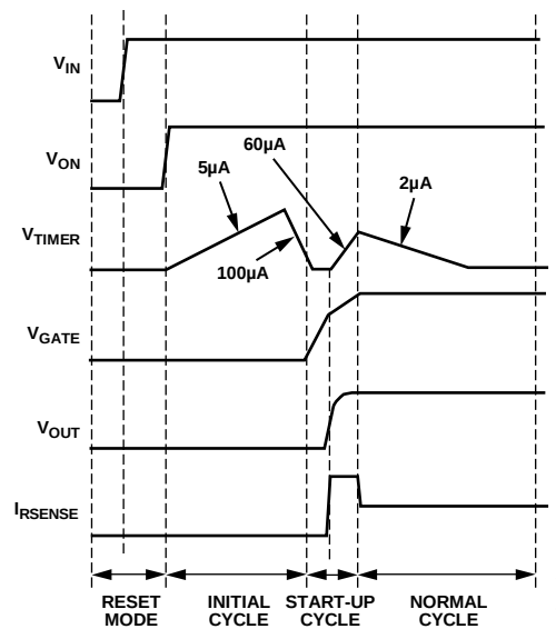
Figure 34. Power-Up into Capacitor
