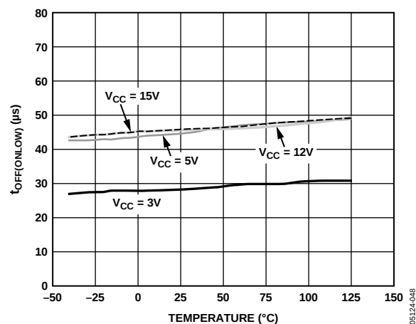
Figure 25. t_{\text{OFF}}(\text{ONLOW}) vs. Temperature
