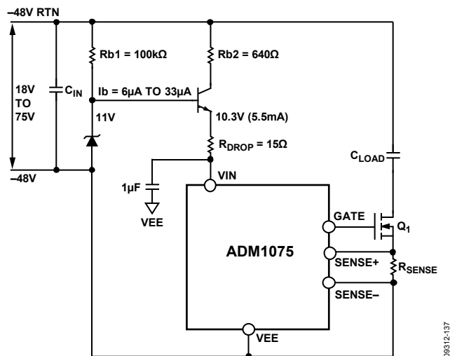
Figure 43. Wide Input Supply Range
