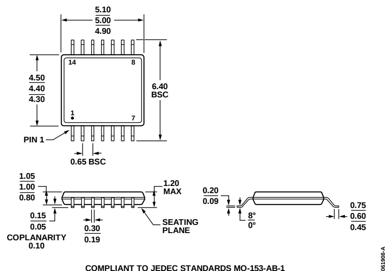
COMPLIANT TO JEDEC STANDARDS MO-153-AB-1 Figure 49. 14-Lead Thin Shrink Small Outline Package [TSSOP] (RU-14) Dimensions shown in millimeters
