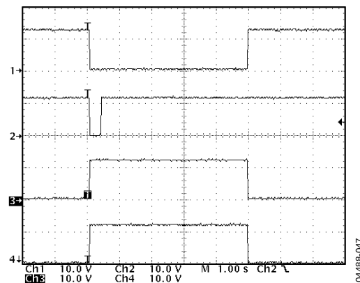
Figure 47. Timing Waveforms Associated with a \overline{\text{RESTART}} Event (Ch1 = GATE; Ch2 = \overline{\text{RESTART}} ; Ch3 = \overline{\text{PWRGD}} ; Ch4 = \overline{\text{SPLYGD}} )
