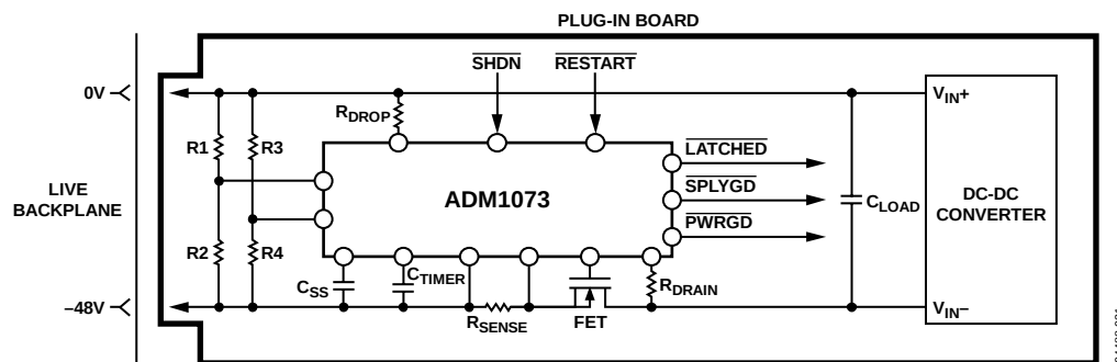
Figure 31. ADM1073 Topology
