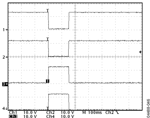
Figure 46. Timing Waveforms Associated with a \overline{\text{RESET}} Event (Ch1 = GATE; Ch2 = \overline{\text{SHDN}} ; Ch3 = \overline{\text{PWRGD}} ; Ch4 = \overline{\text{SPLYGD}} )
