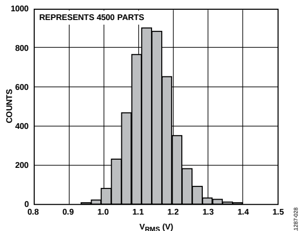
Figure 28. Distribution of V_{RMS} , P_{IN} = -45 dBm, 900 MHz
