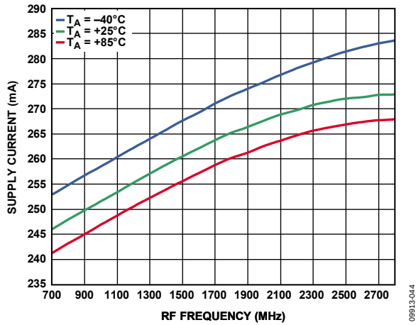
Figure 53. Supply Current vs. RF Frequency at 3.6 V
