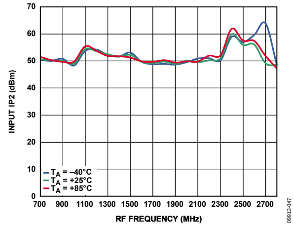
Figure 56. Input IP2 vs. RF Frequency at 3.6 V
