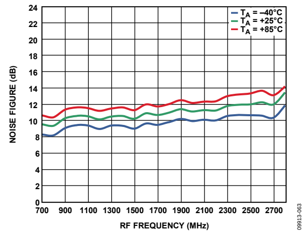
Figure 58. SSB Noise Figure vs. RF Frequency at 3.6 V
