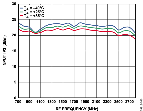
Figure 55. Input IP3 vs. RF Frequency at 3.6 V
