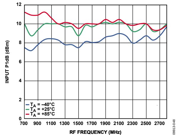
Figure 57. Input P1dB vs. RF Frequency at 3.6 V
