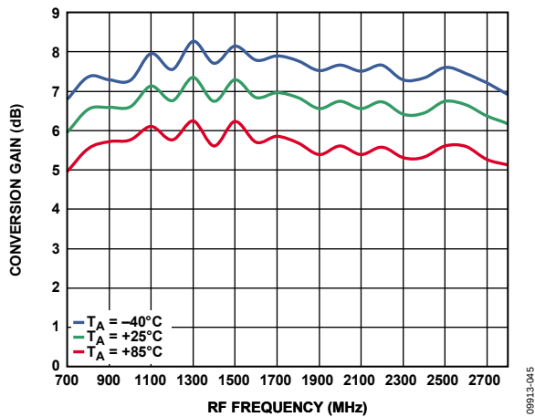
Figure 54. Power Conversion Gain vs. RF Frequency at 3.6 V
