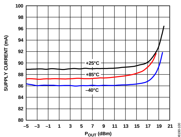
Figure 15. Supply Current vs. P_{OUT} and Temperature V_{CC} = 5\text{ V}
