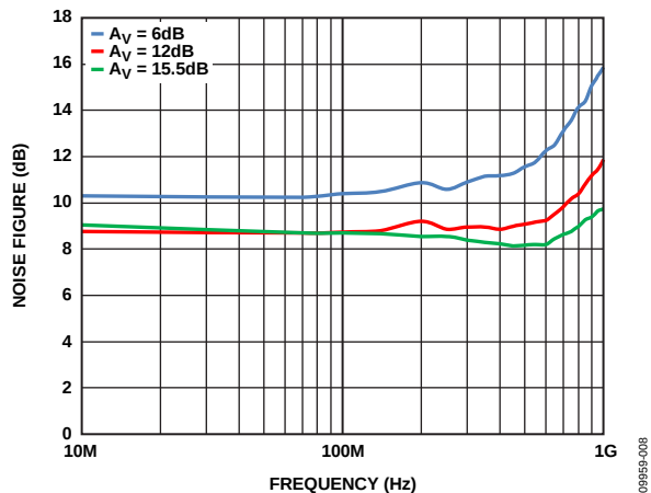
Figure 9. Noise Figure vs. Frequency at A_V = 6 dB, A_V = 12 dB, and A_V = 15.5 dB, V_{POS} = 5 V
