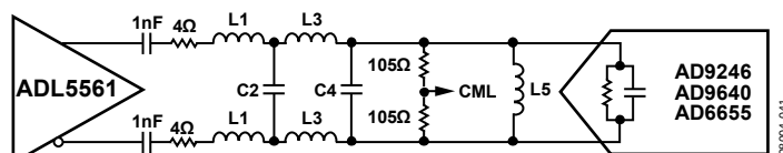
Figure 40. Narrow-Band IF Sampling Solution for an Unbuffered ADC Application
