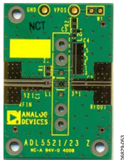
Figure 55. Evaluation Board Layout (Top View)
