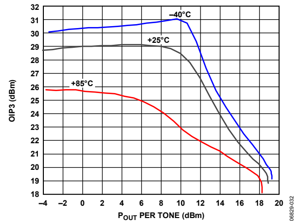
Figure 32. OIP3 vs. Output Power ( P_{OUT} ) and Temperature
