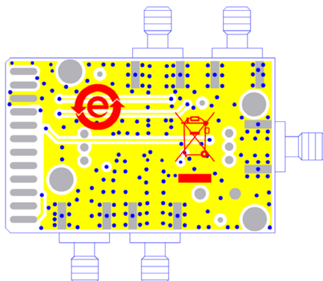
Figure 20. Layout of Evaluation Board, Circuit Side
