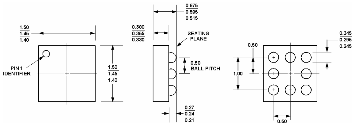
Figure 21. 8-Bump Wafer Level Chip Scale Package [WLCSP] (TBD)
