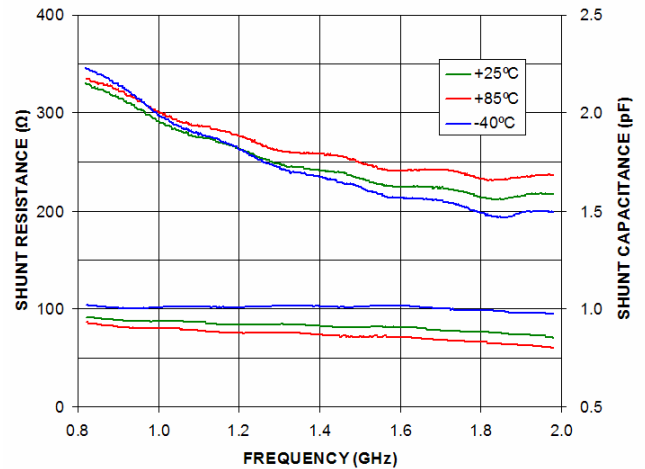
Figure 7. Input Impedance vs. Frequency, Supply 3.0 V, Temperatures -40^\circ\text{C} , +25^\circ\text{C} , and +85^\circ\text{C}
