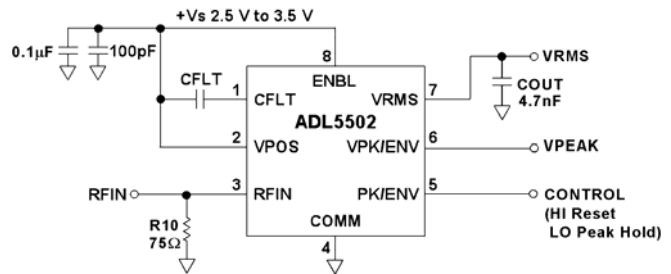
Figure 17. Basic Connections for ADL5502
