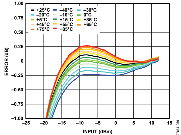
Figure 59. VRMS Typical Drift at 1.9 GHz for Various Temperatures
