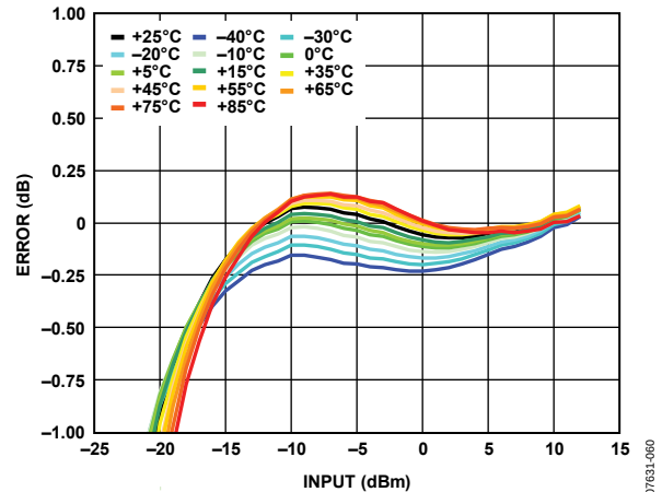
Figure 60. PEAK Typical Drift at 1.9 GHz for Various Temperatures
