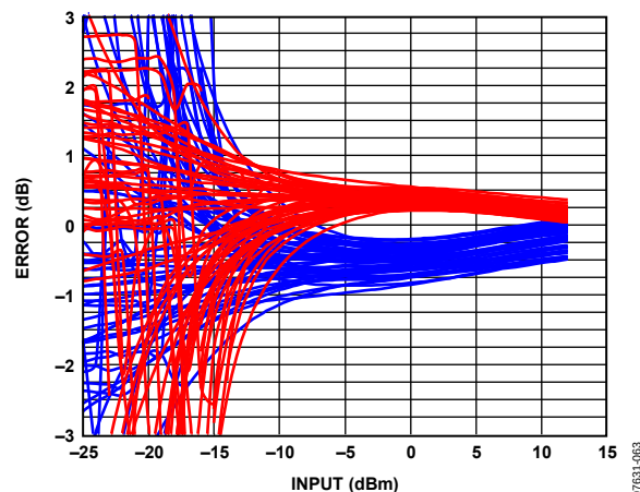
Figure 63. VRMS Output Delta from +25°C Output Voltage for 50 Devices at -40°C and +85°C, Frequency 6000 MHz, Supply 3.0 V
