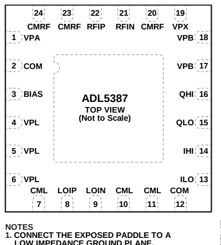
Figure 2. Pin Configuration
