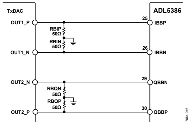
Figure 46. Interface Between AD9788 and ADL5386 with 50 \Omega Resistors to Ground to Establish the 500 mV DC Bias for the ADL5386 Baseband Inputs
