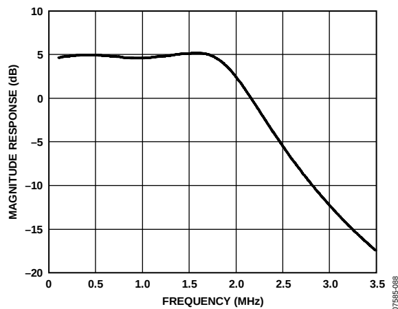
Figure 93. Sixth-Order Baseband Filter Response
