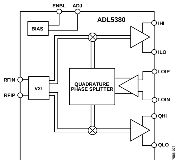
Figure 76. Block Diagram
