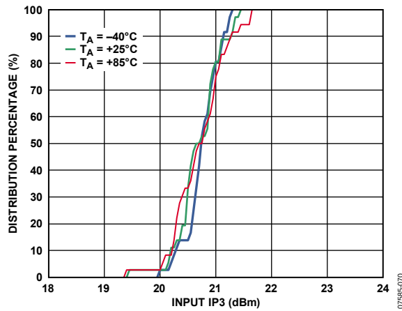
Figure 70. IIP3 Distributions
