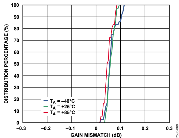
Figure 60. IQ Gain Mismatch Distributions
