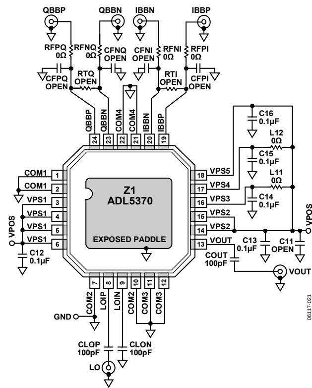
Figure 36. ADL5370 Evaluation Board Schematic
