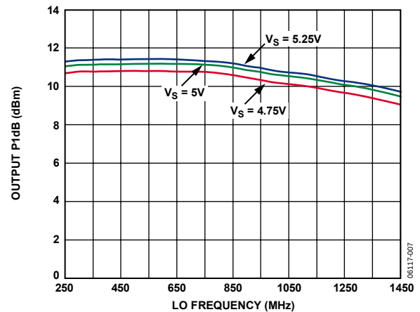
Figure 7. SSB Output 1 dB Compression Point (OP1dB) vs. f_{\text{LO}} and Supply
