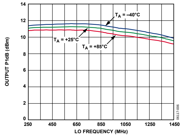
Figure 6. SSB Output 1 dB Compression Point (OP1dB) vs. f_{\text{LO}} and Temperature
