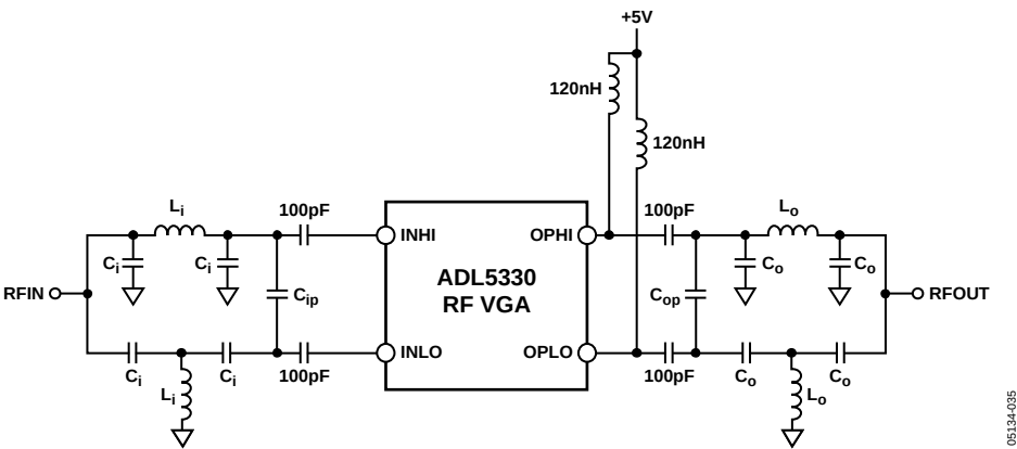
Figure 35. Differential Operation with Discrete LC Baluns
