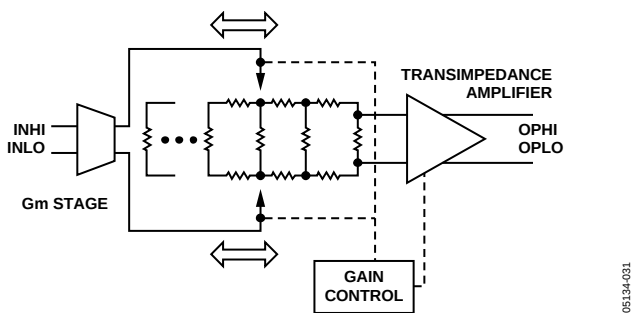
Figure 31. Simplified Schematic
