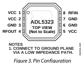
Figure 3. Pin Configuration
