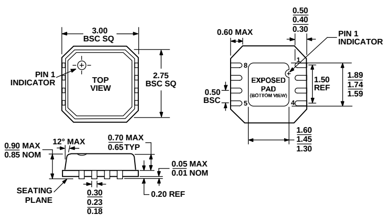
Figure 20. 8-Lead Lead Frame Chip Scale Package [LFCSP_VD] 3 mm x 3 mm Body, Very Thin, Dual Lead (CP-8-2) Dimensions shown in millimeters
