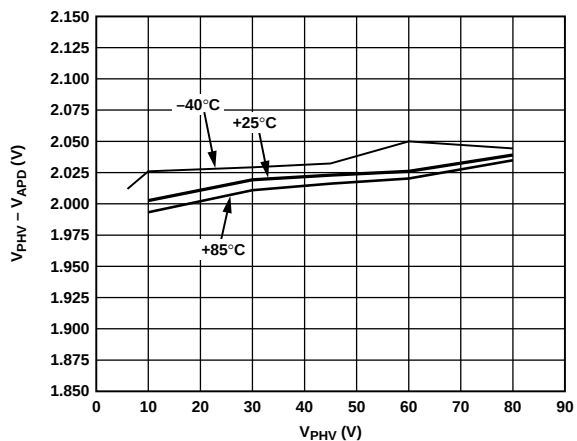
Figure 5. V_{APD} Supply Tracking Offset vs. V_{PHV} for Multiple Temperatures
