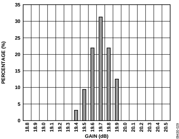
Figure 30. AMP: Gain Distribution at 2140 MHz
