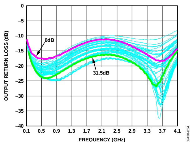
Figure 15. DSA: Output Return Loss vs. Frequency, All States
