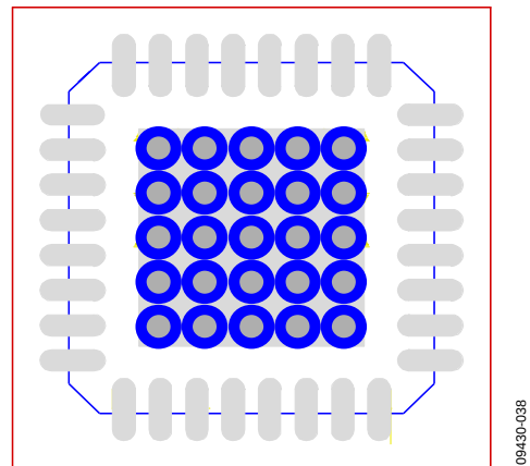
Figure 40. Exposed Pad with Thermal Via Distribution
