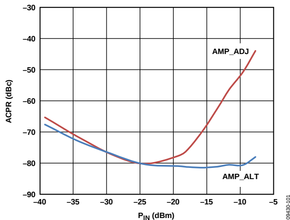
Figure 39. Single Carrier WCDMA Adjacent Channel Power Ratio vs. Input Power at Amplifier, 2140 MHz
