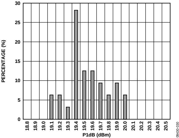
Figure 31. AMP: P1dB Distribution at 2140 MHz
