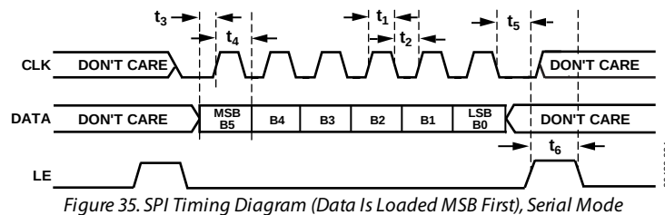
Figure 35. SPI Timing Diagram (Data Is Loaded MSB First), Serial Mode
