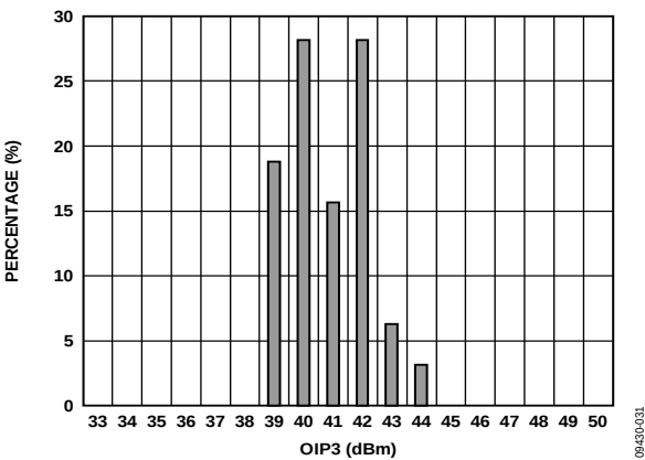
Figure 32. AMP: OIP3 Distribution at 2140 MHz
