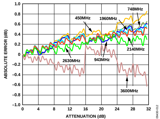
Figure 13. DSA: Absolute Error vs. Attenuation
