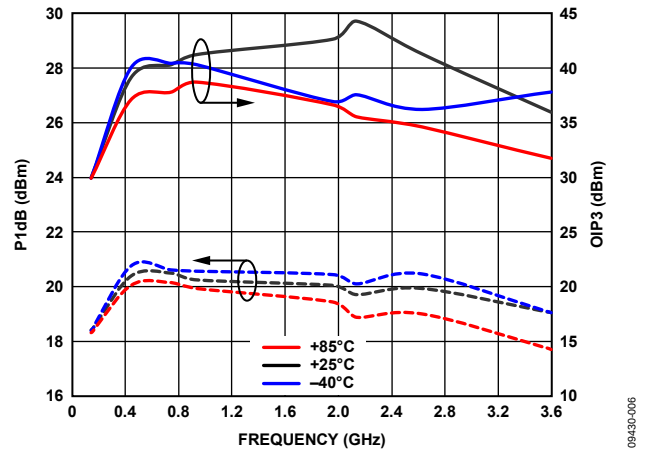
Figure 6. AMP: OIP3 at P_{OUT} = 4 dBm/Tone and P1dB vs. Frequency and Temperature
