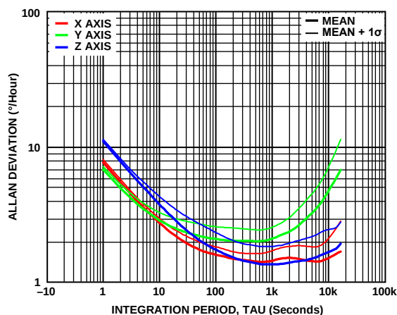
Figure 7. Gyroscope Allan Deviation, T_C = 25^\circ\text{C} , ADIS16507-1, Plot Taken After 10 Hours of Settling Time
