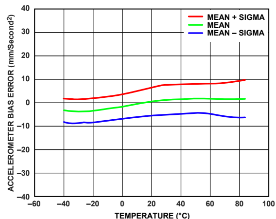
Figure 25. Accelerometer Bias Error vs. Temperature, All Axes, Hot to Cold
