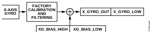
Figure 57. User Calibration Signal Path, Gyroscopes
