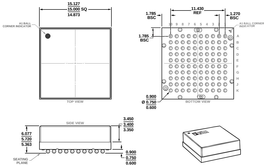
Figure 67. 100-Ball Ball Grid Array Module [BGA] (ML-100-1)
