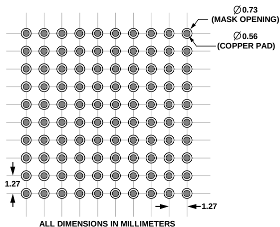
Figure 63. Recommend PCB Pattern, Solder Mask Defined Pads
