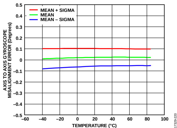
Figure 20. Axis to Axis Gyroscope Misalignment Error vs. Temperature, All Axes, Cold to Hot, ADIS16507-2
