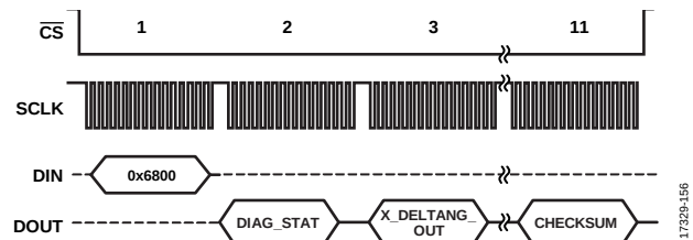
Figure 44. Burst Read Sequence with BURST_SEL = 1
