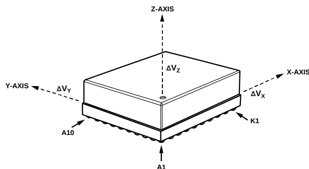
Figure 55. Delta Velocity Axis and Polarity Assignments
