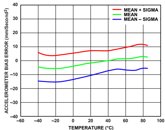
Figure 24. Accelerometer Bias Error vs. Temperature, All Axes, Cold to Hot
