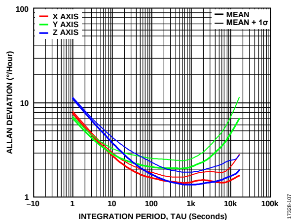
Figure 7. Gyroscopic Allan Deviation, T_C = 25^\circ\text{C} , ADIS16505-1, Plot Taken After 10 Hours of Settling Time
