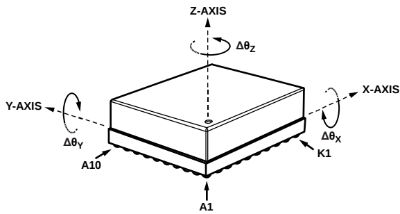
Figure 52. Delta Angle Axis and Polarity Assignments
