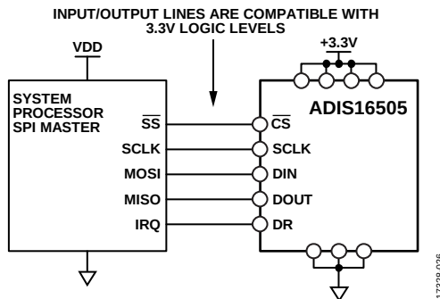
Figure 34. Electrical Connection Diagram
