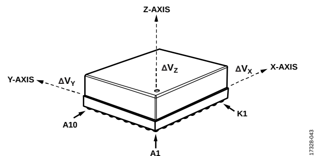
Figure 54. Delta Velocity Axis and Polarity Assignments
