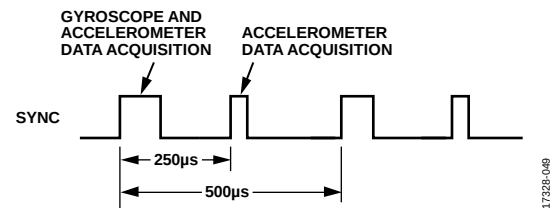
Figure 29. Sync Output Signal, Register MSC_CTRL, Bits[3:2] = 11
