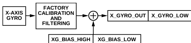
Figure 56. User Calibration Signal Path, Gyroscopes
