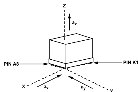
Figure 38. Accelerometer Axis and Polarity Assignments
