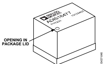
Figure 50. Pressure Relief Hole
