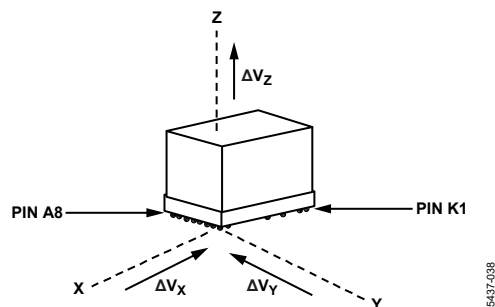
Figure 42. Delta Velocity Axis and Polarity Assignments
