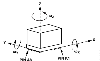
Figure 36. Gyroscope Axis and Polarity Assignments
