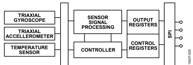
Figure 24. Basic Operation of the ADIS16477
