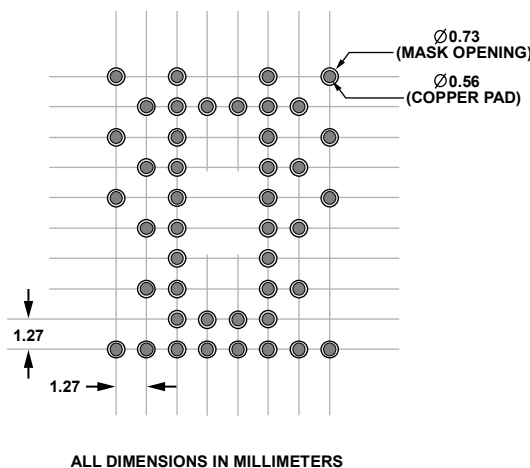
Figure 51. Recommend PCB Pattern, Solder Mask Defined Pads
