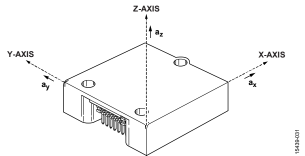
Figure 39. Accelerometer Axis and Polarity Assignments
