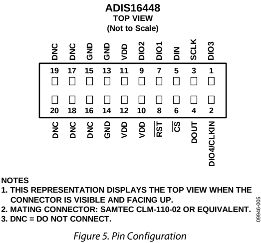
Figure 5. Pin Configuration
